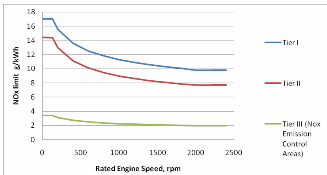
Figure 3. NO x emission limits
