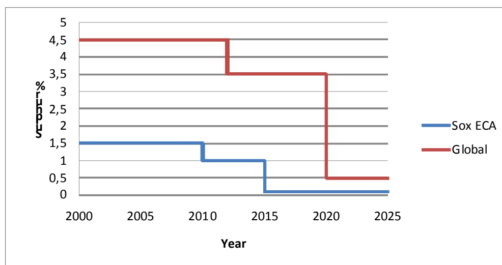
Figure 2. Sulphur Limit in Fuel
